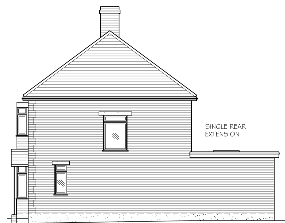
PROPOSED SIDE (EAST-NORTH) ELEVATION 1:100
