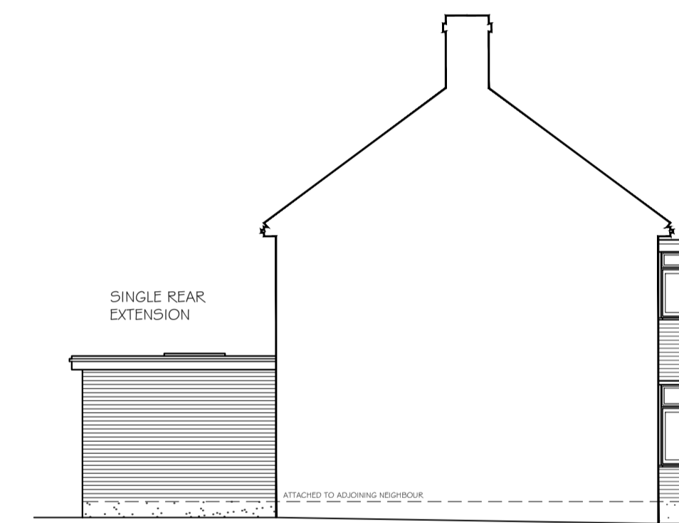
PROPOSED SIDE (SOUTH-WEST) ELEVATION 1:100
