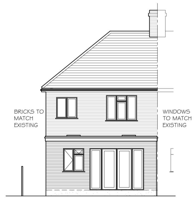
PROPOSED REAR (NORTH-WEST) ELEVATION 1:100
